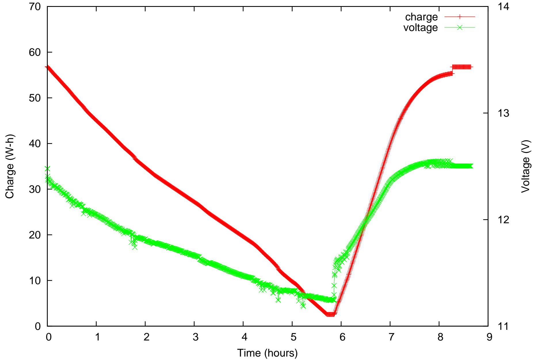
SANYO 42T4649 (design charge 84.24 W-h) in a Lenovo X200s model 7466-3JU
